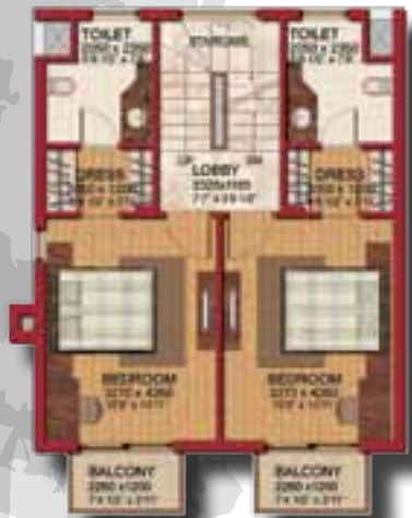
FIRST LOWER GROUND FLOOR PLAN
